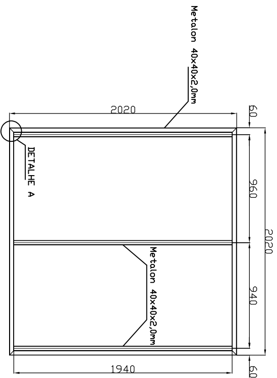
VISTA FRONTAL
